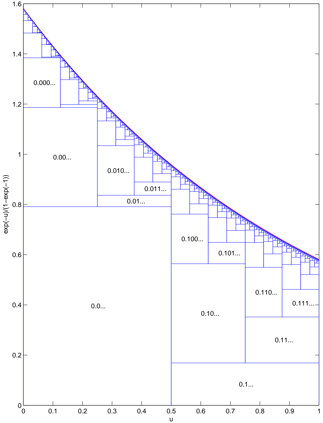
Exact binary sampling of exponential distribution
